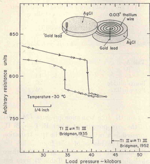
Fig. 4. The transition T\text{I II} \rightleftharpoons T\text{I III} as shown by the change in electrical resistance of a thallium wire in an AgCl cell.
